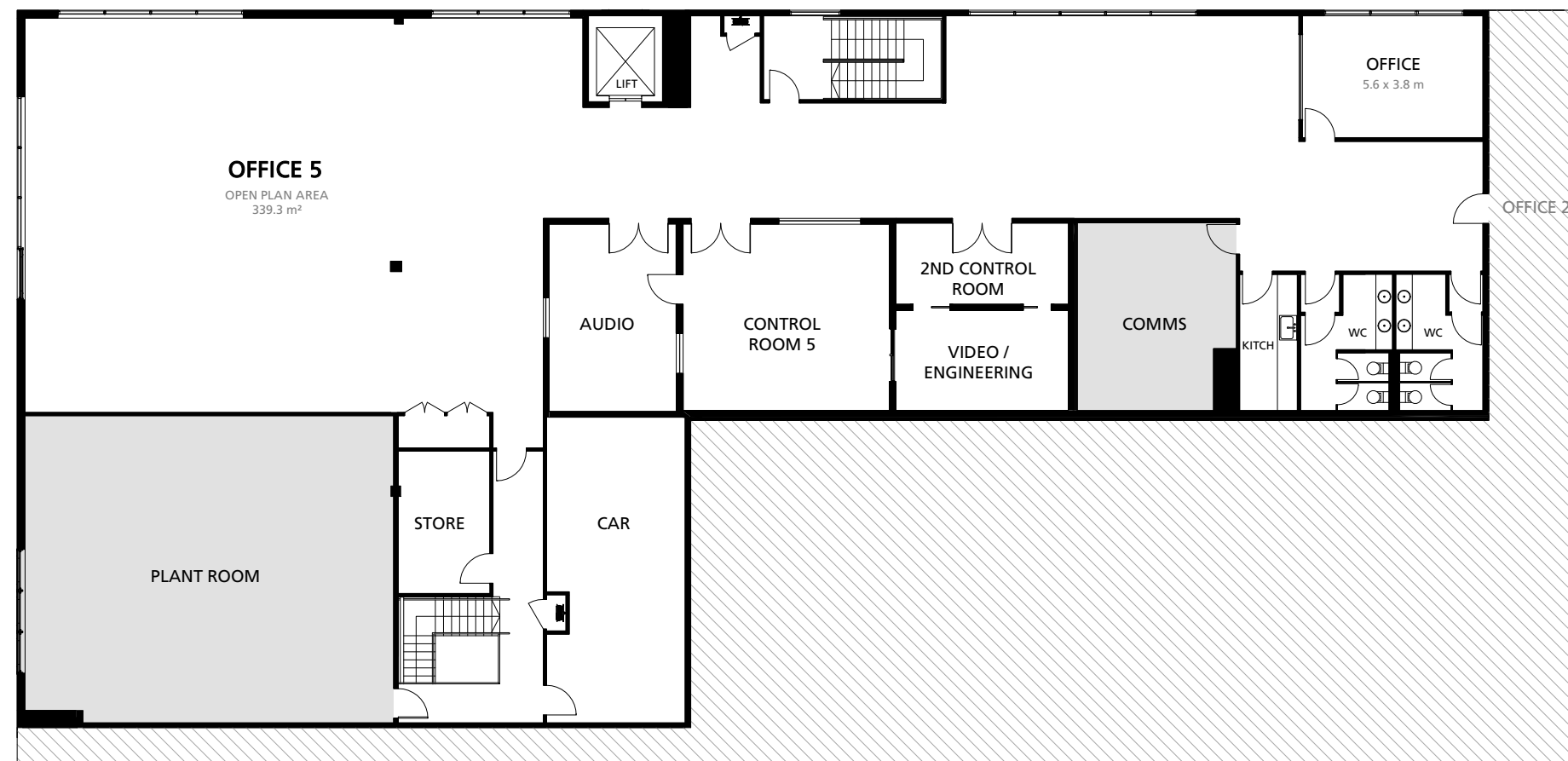
2 UPPER LEVEL PLAN
